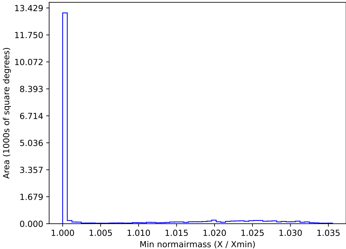
weather_cloudso4v3.4_10yrs WFD r band: Min normairmass
