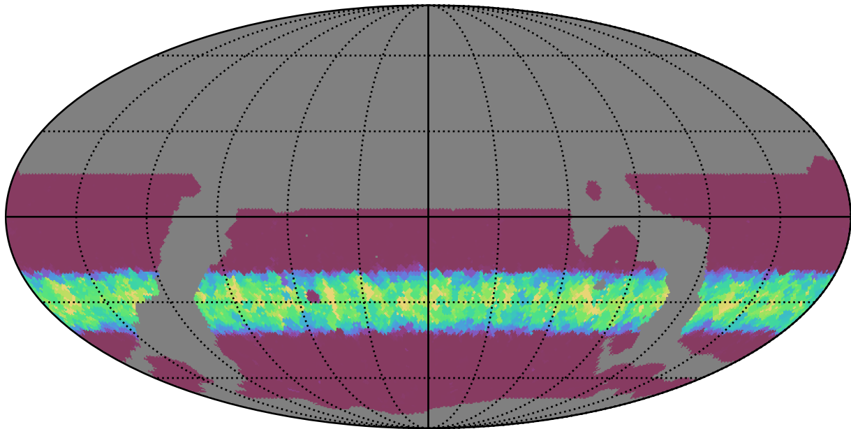
weather_cloudso4v3.4_10yrs WFD g band: Min normairmass
