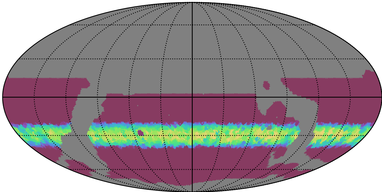
weather_cloudso4v3.4_10yrs WFD all bands: Min normairmass
