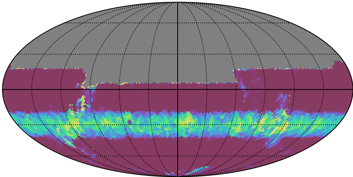
weather_cloudso4v3.4_10yrs All sky u band: Min normairmass
