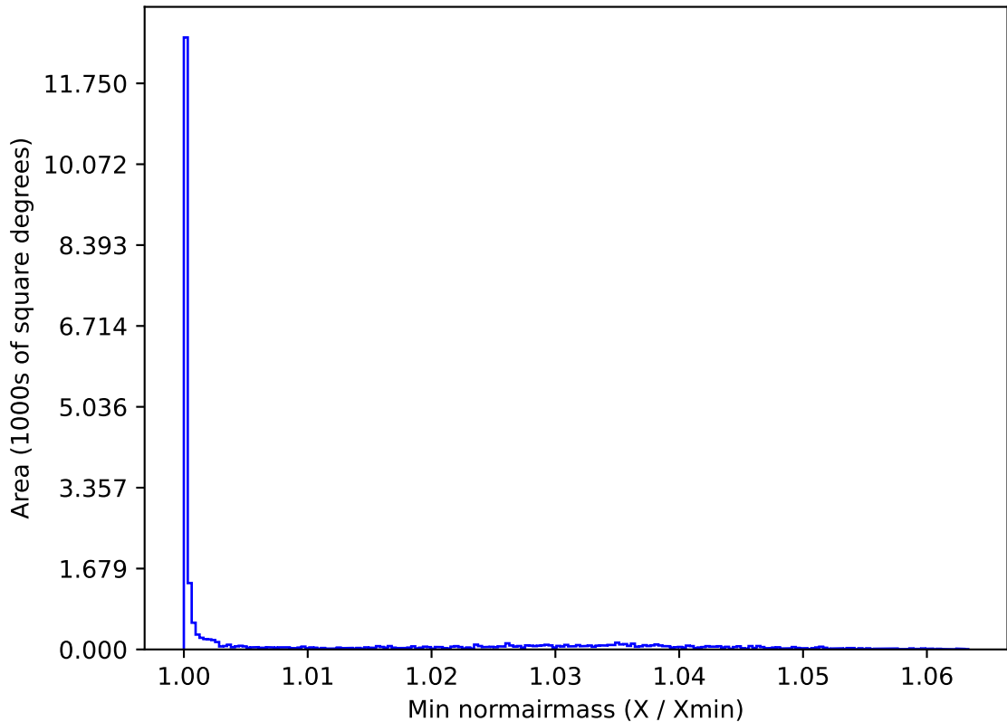
weather_cloudso4v3.4_10yrs All sky u band: Min normairmass
