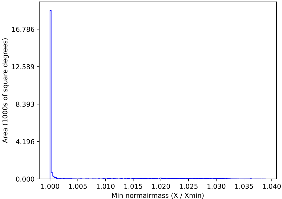
weather_cloudso4v3.4_10yrs All sky r band: Min normairmass
