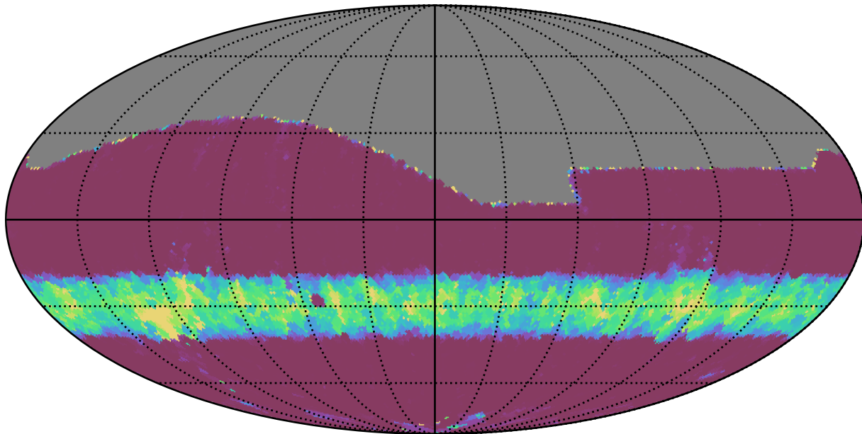
weather_cloudso4v3.4_10yrs All sky g band: Min normairmass
