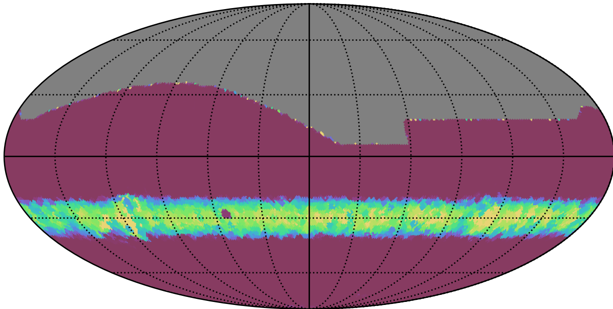
weather_cloudso4v3.4_10yrs All sky all bands: Min normairmass
