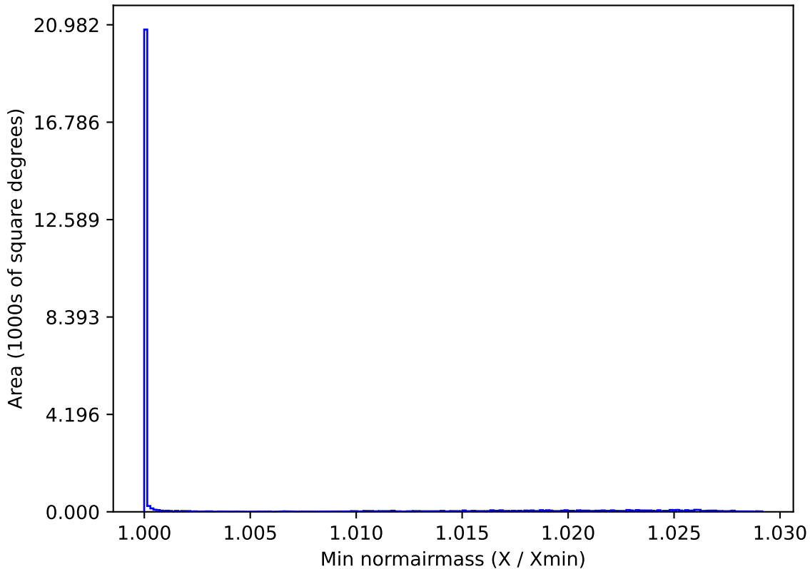
weather_cloudso4v3.4_10yrs All sky all bands: Min normairmass
