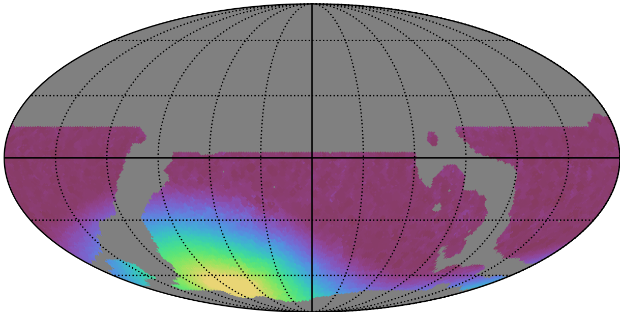
weather_cloudso4v3.4_10yrs WFD z band: Min moonDistance
