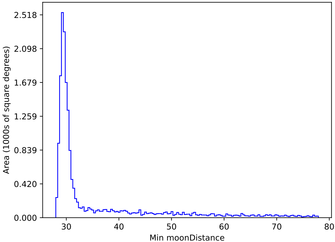
weather_cloudso4v3.4_10yrs WFD z band: Min moonDistance
