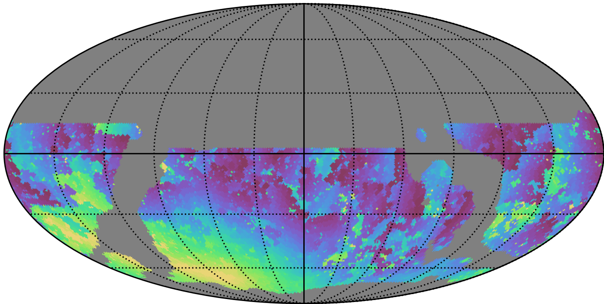
weather_cloudso4v3.4_10yrs WFD u band: Min moonDistance
