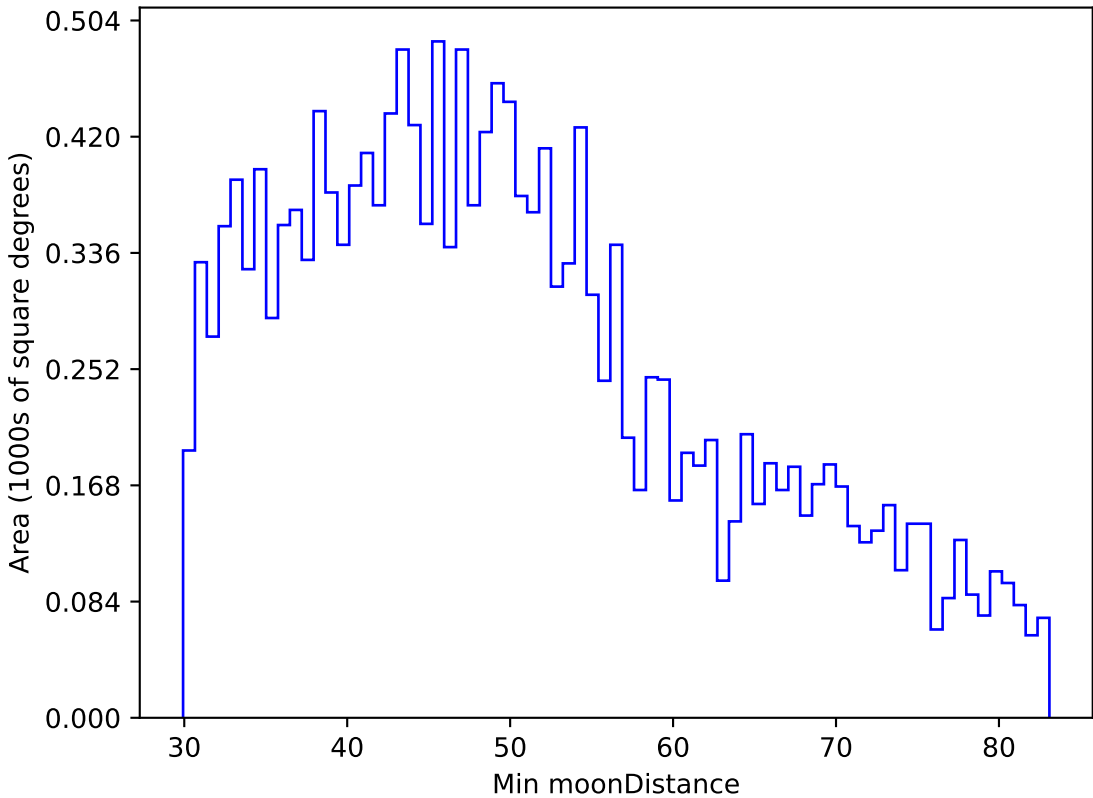
weather_cloudso4v3.4_10yrs WFD u band: Min moonDistance
