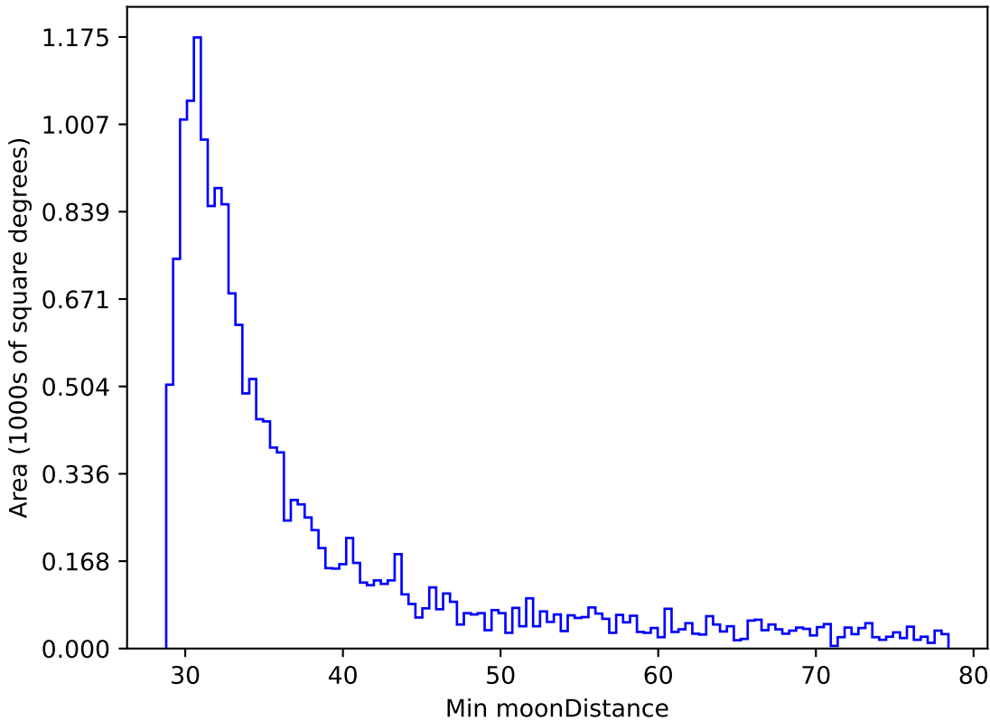
weather_cloudso4v3.4_10yrs WFD r band: Min moonDistance
