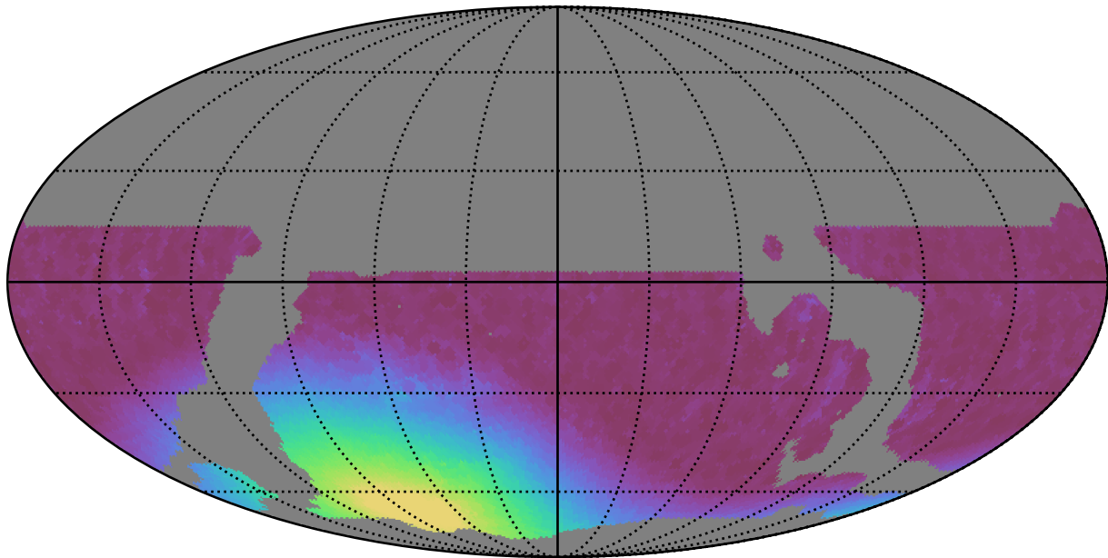
weather_cloudso4v3.4_10yrs WFD i band: Min moonDistance
