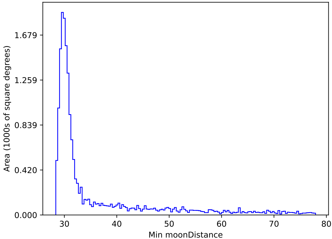
weather_cloudso4v3.4_10yrs WFD i band: Min moonDistance
