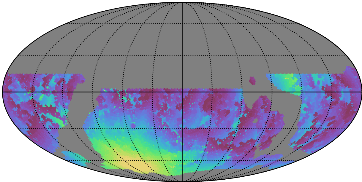
weather_cloudso4v3.4_10yrs WFD g band: Min moonDistance
