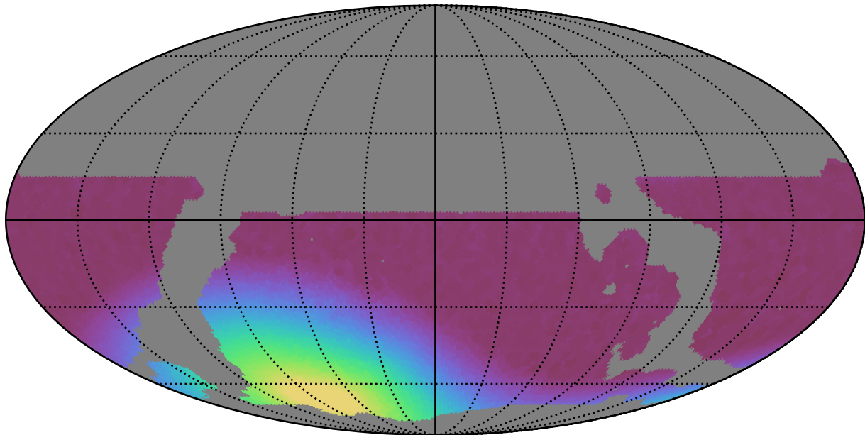
weather_cloudso4v3.4_10yrs WFD all bands: Min moonDistance
