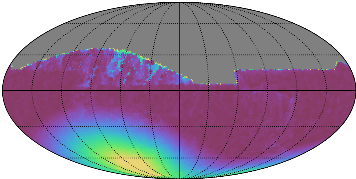
weather_cloudso4v3.4_10yrs All sky z band: Min moonDistance
