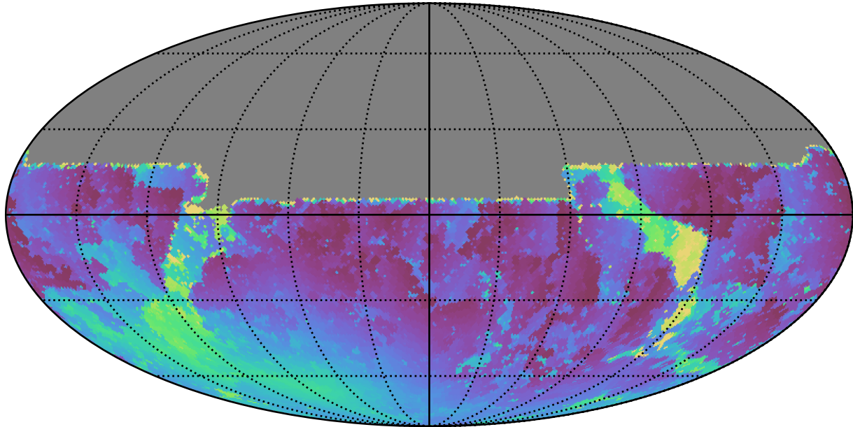
weather_cloudso4v3.4_10yrs All sky u band: Min moonDistance
