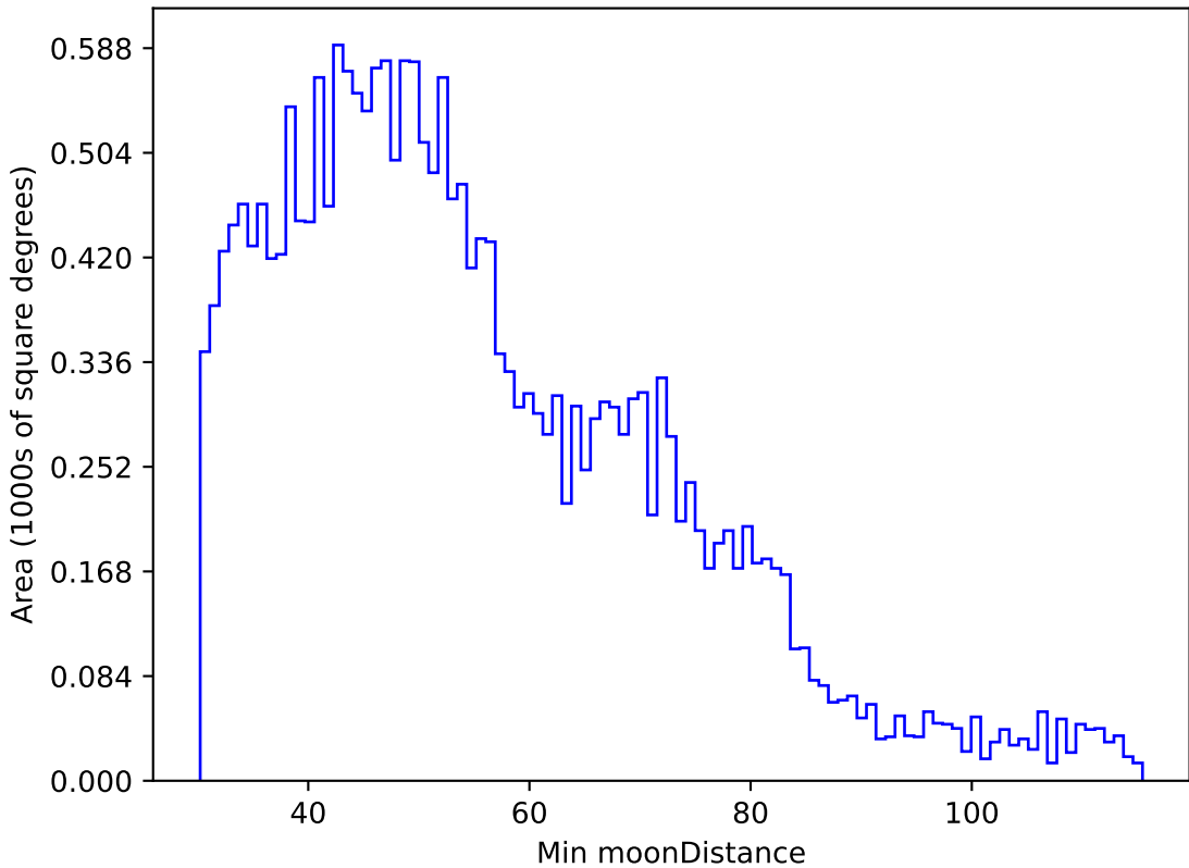
weather_cloudso4v3.4_10yrs All sky u band: Min moonDistance
