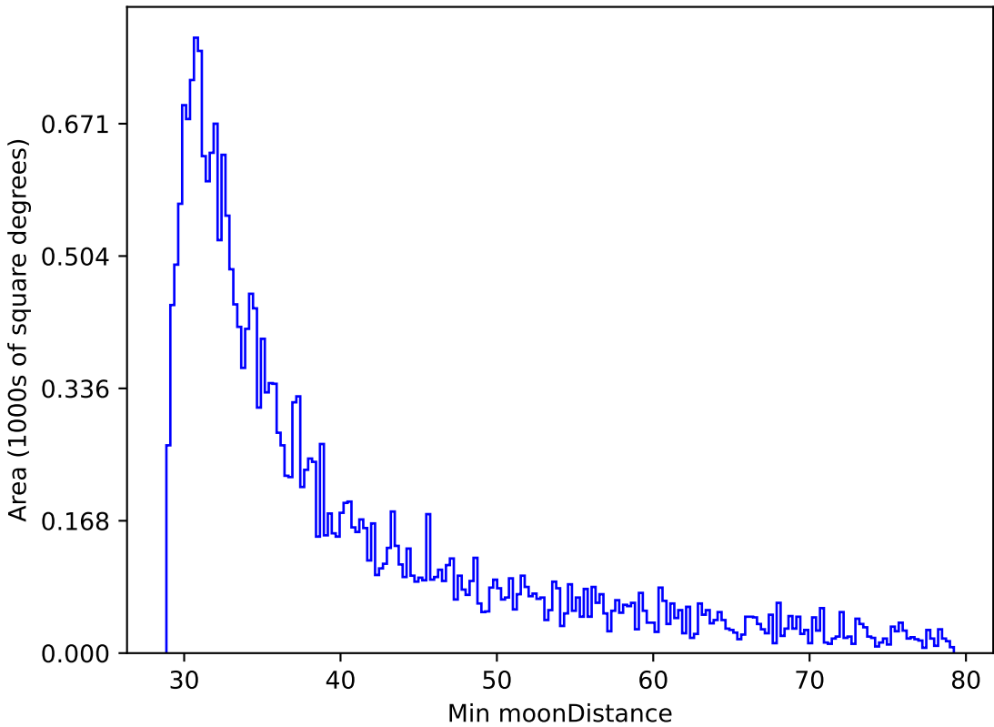
weather_cloudso4v3.4_10yrs All sky r band: Min moonDistance
