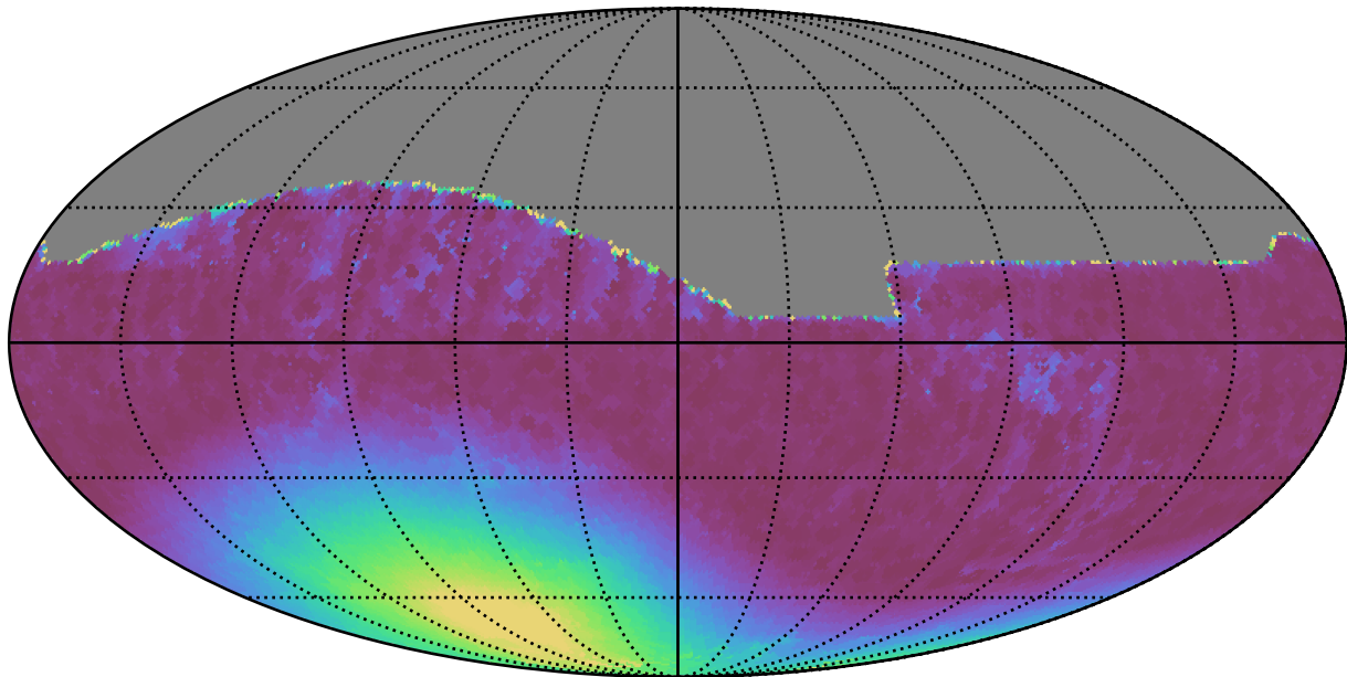
weather_cloudso4v3.4_10yrs All sky i band: Min moonDistance
