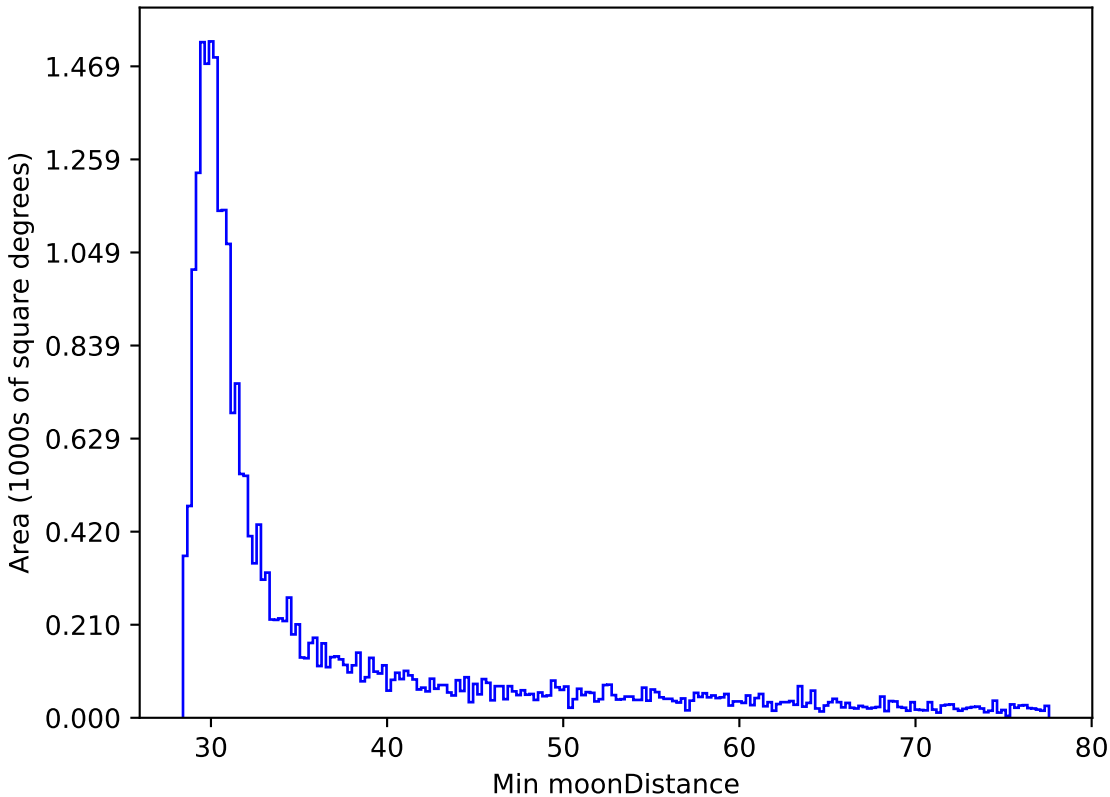
weather_cloudso4v3.4_10yrs All sky i band: Min moonDistance
