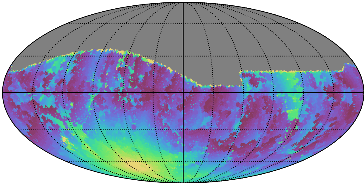
weather_cloudso4v3.4_10yrs All sky g band: Min moonDistance
