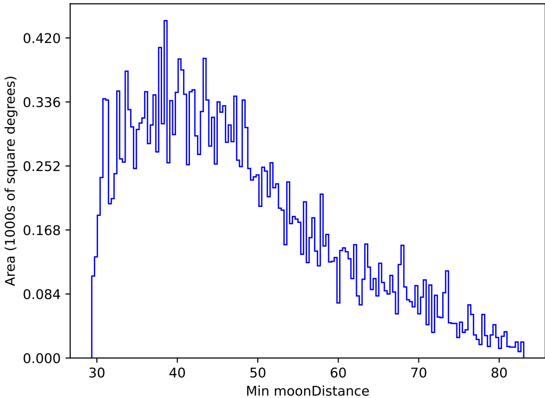
weather_cloudso4v3.4_10yrs All sky g band: Min moonDistance
