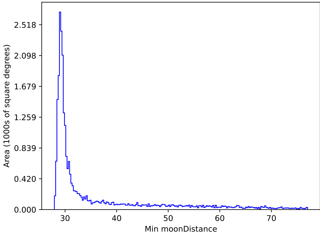
weather_cloudso4v3.4_10yrs All sky all bands: Min moonDistance
