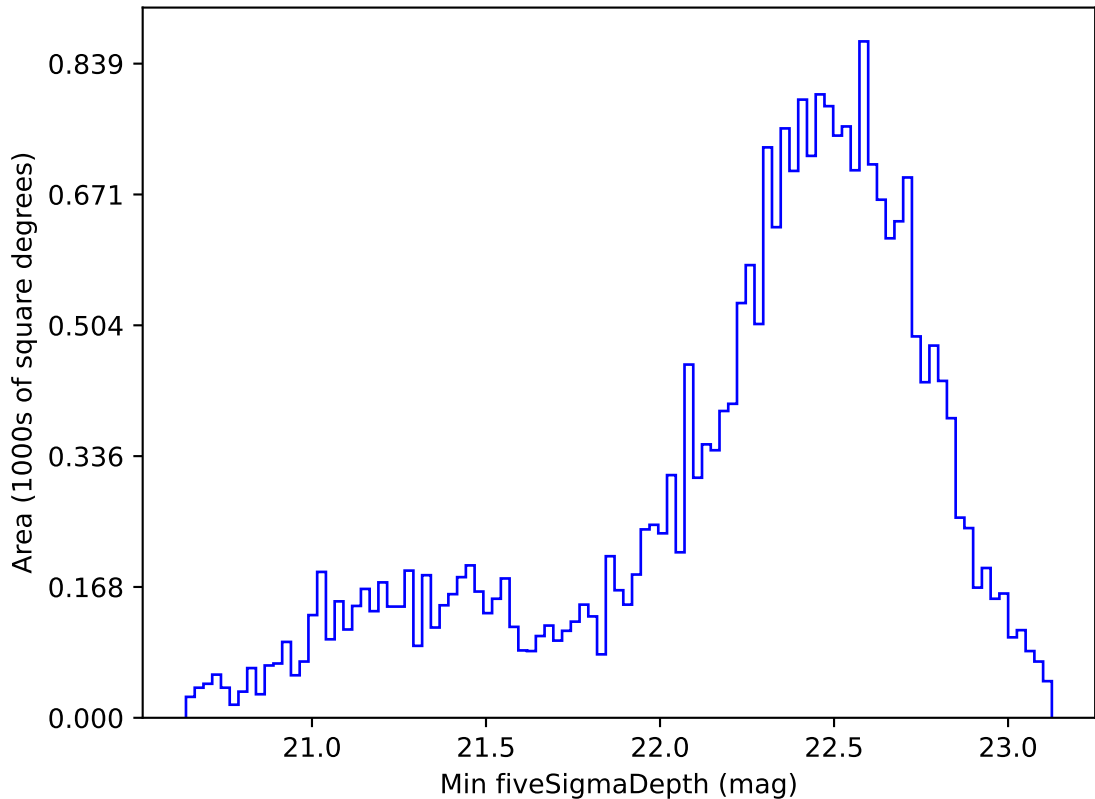
weather_cloudso4v3.4_10yrs Yr 1 z band: Min fiveSigmaDepth
