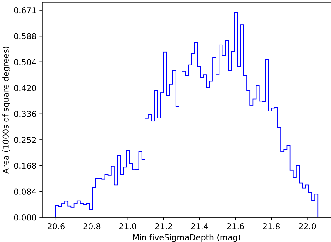
weather_cloudso4v3.4_10yrs Yr 1 y band: Min fiveSigmaDepth
