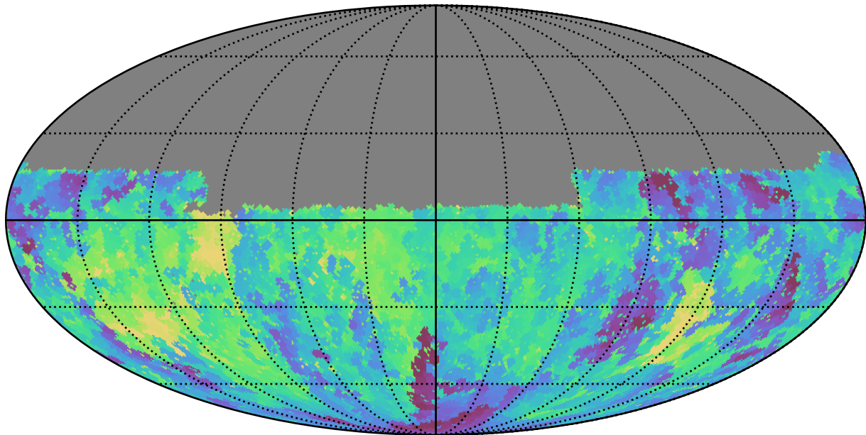
weather_cloudso4v3.4_10yrs Yr 1 u band: Min fiveSigmaDepth
