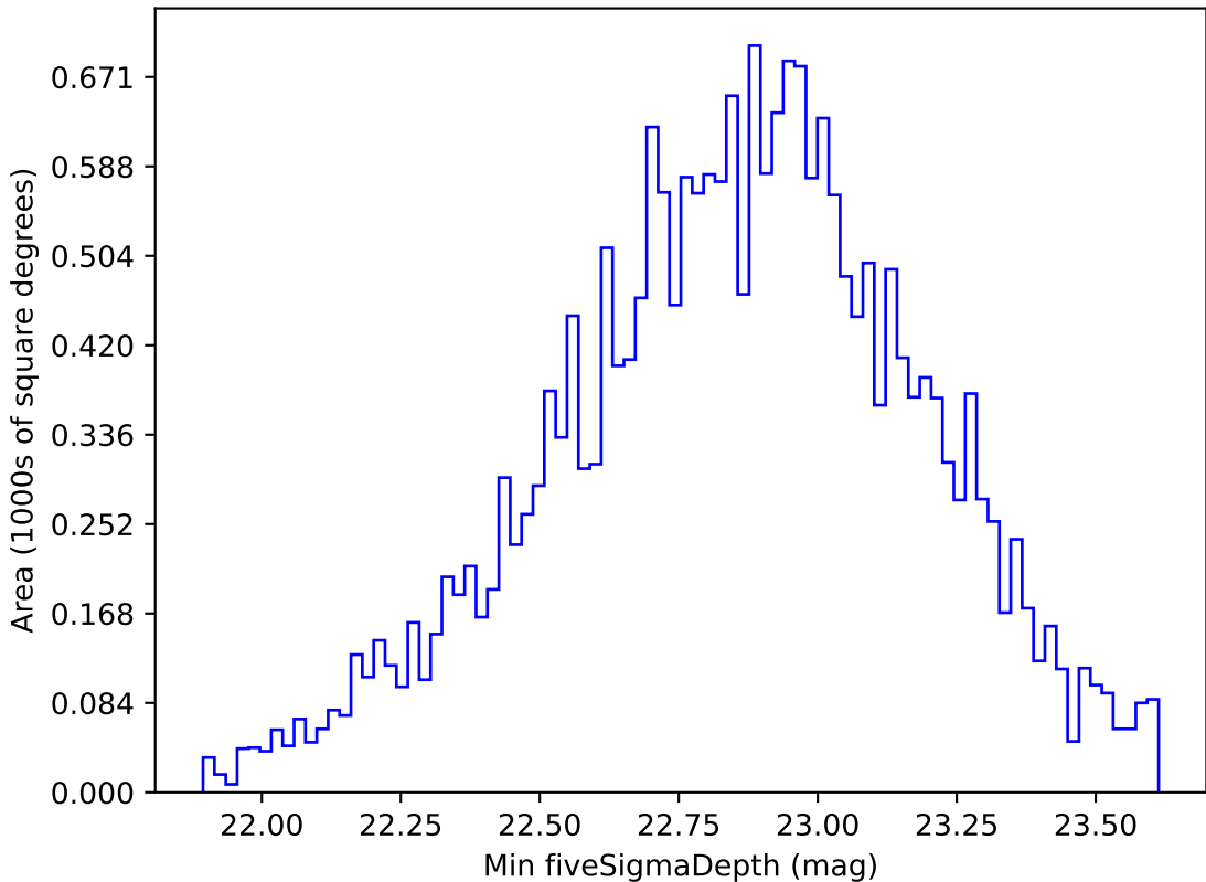
weather_cloudso4v3.4_10yrs Yr 1 u band: Min fiveSigmaDepth
