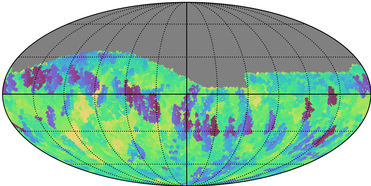
weather_cloudso4v3.4_10yrs Yr 1 i band: Min fiveSigmaDepth
