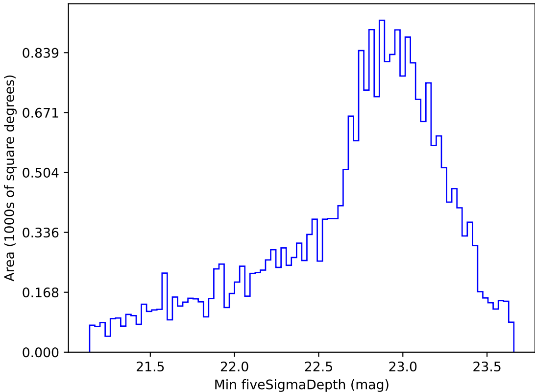
weather_cloudso4v3.4_10yrs Yr 1 i band: Min fiveSigmaDepth
