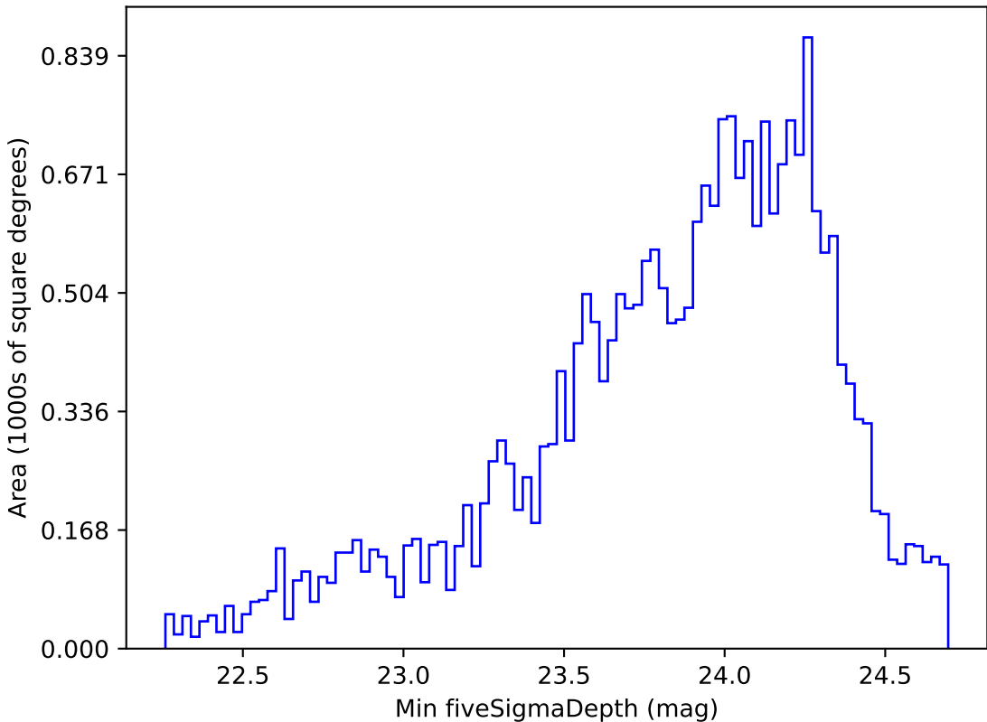
weather_cloudso4v3.4_10yrs Yr 1 g band: Min fiveSigmaDepth
