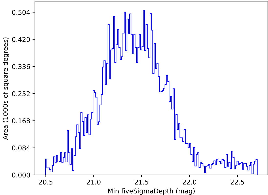
weather_cloudso4v3.4_10yrs Yr 1 all bands: Min fiveSigmaDepth
