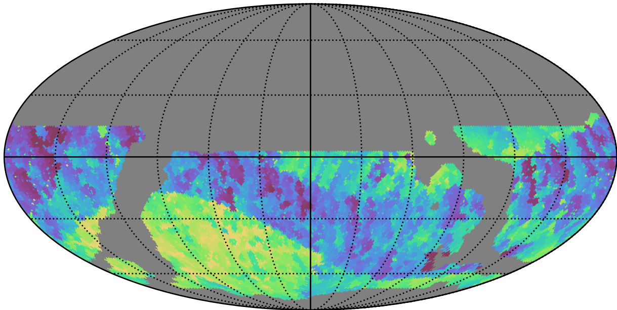
weather_cloudso4v3.4_10yrs WFD z band: Min fiveSigmaDepth
