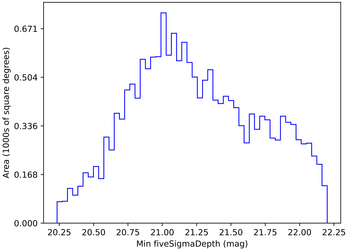
weather_cloudso4v3.4_10yrs WFD z band: Min fiveSigmaDepth
