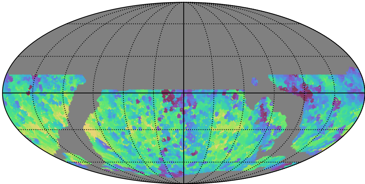
weather_cloudso4v3.4_10yrs WFD y band: Min fiveSigmaDepth
