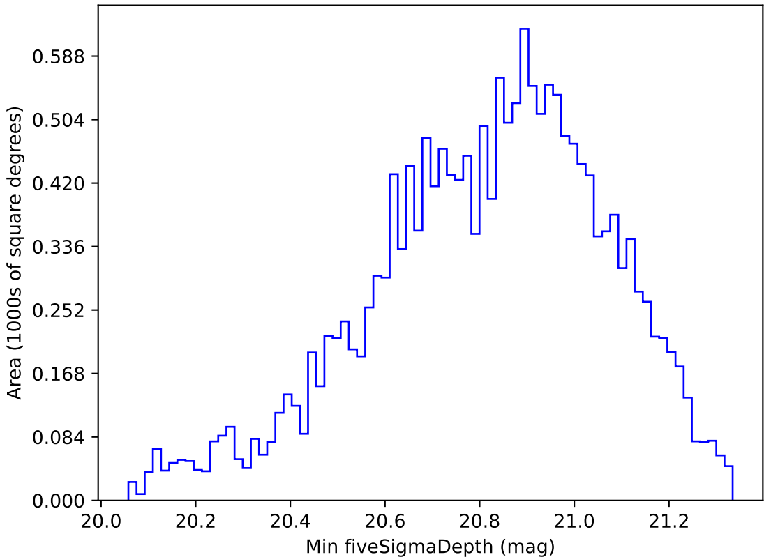
weather_cloudso4v3.4_10yrs WFD y band: Min fiveSigmaDepth
