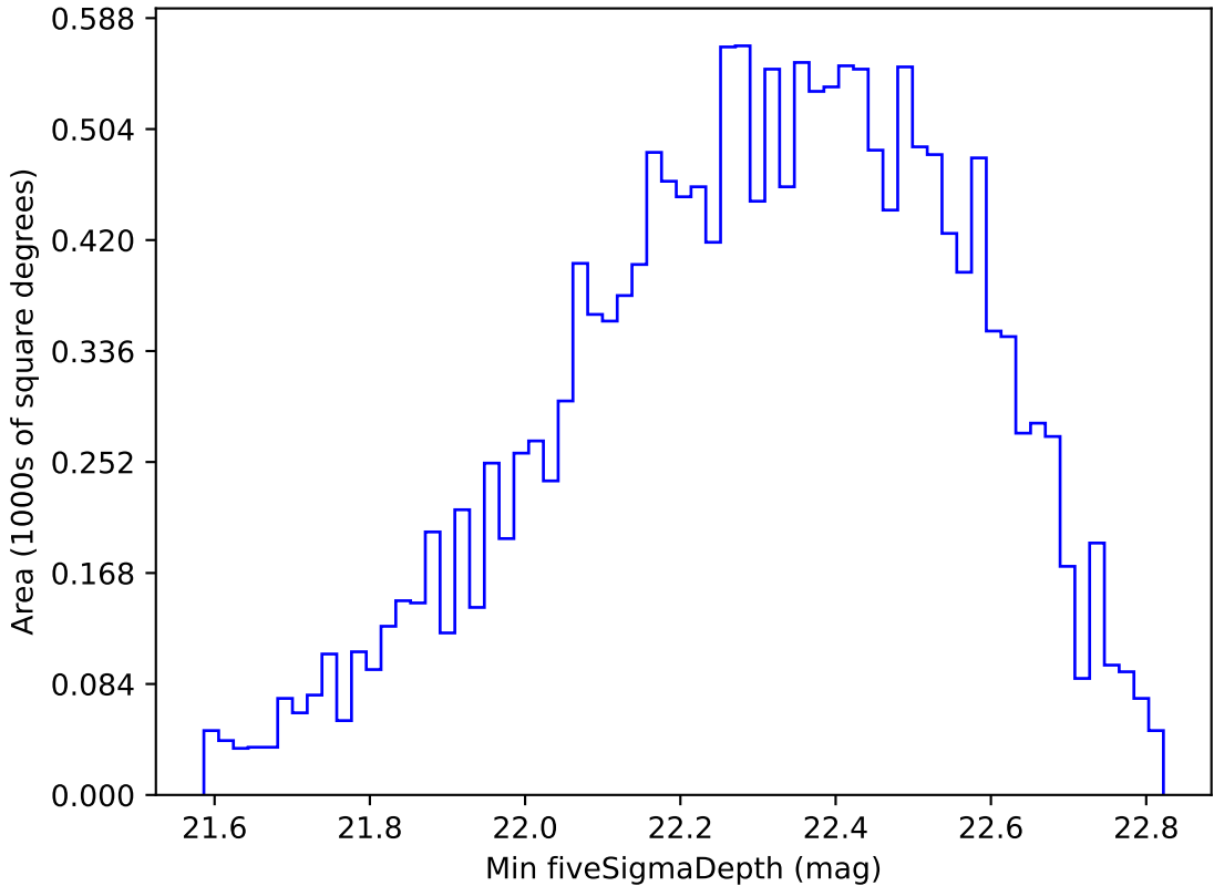
weather_cloudso4v3.4_10yrs WFD u band: Min fiveSigmaDepth
