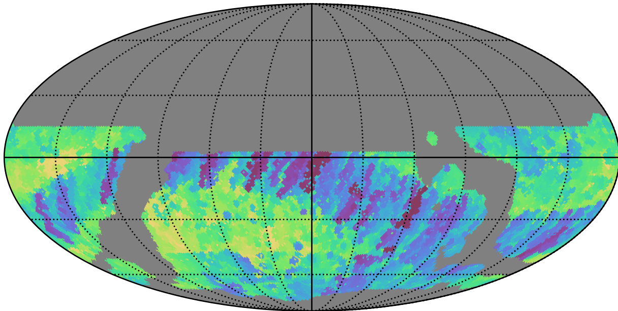
weather_cloudso4v3.4_10yrs WFD r band: Min fiveSigmaDepth
