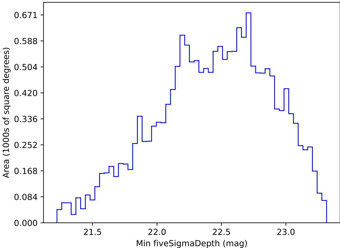
weather_cloudso4v3.4_10yrs WFD r band: Min fiveSigmaDepth
