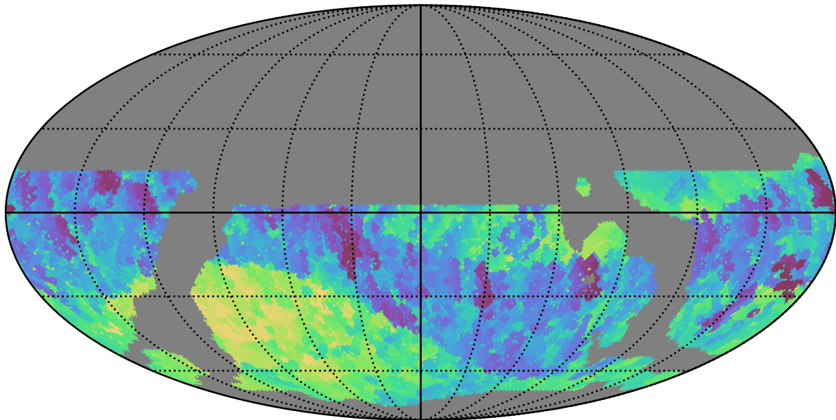
weather_cloudso4v3.4_10yrs WFD i band: Min fiveSigmaDepth
