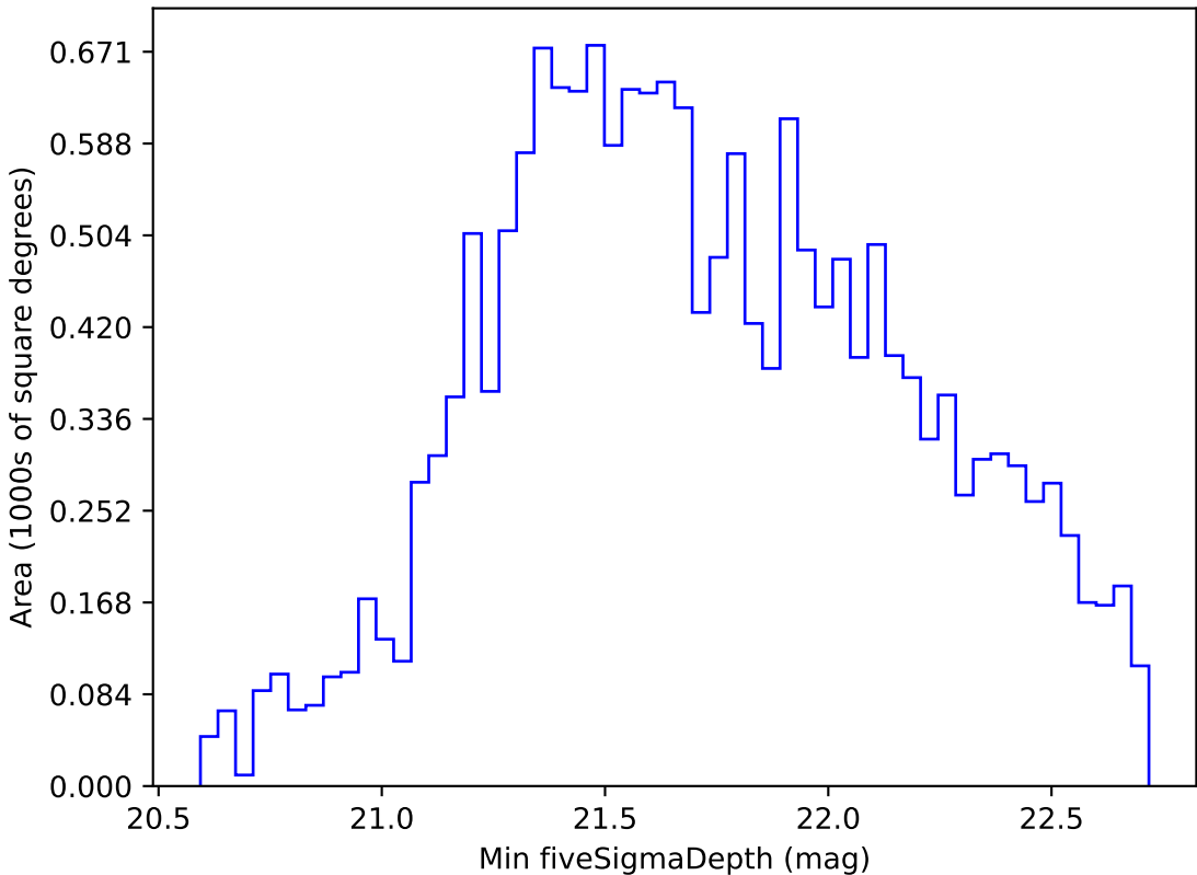
weather_cloudso4v3.4_10yrs WFD i band: Min fiveSigmaDepth
