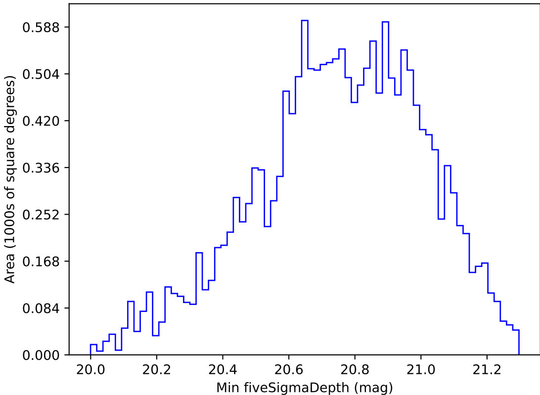
weather_cloudso4v3.4_10yrs WFD all bands: Min fiveSigmaDepth
