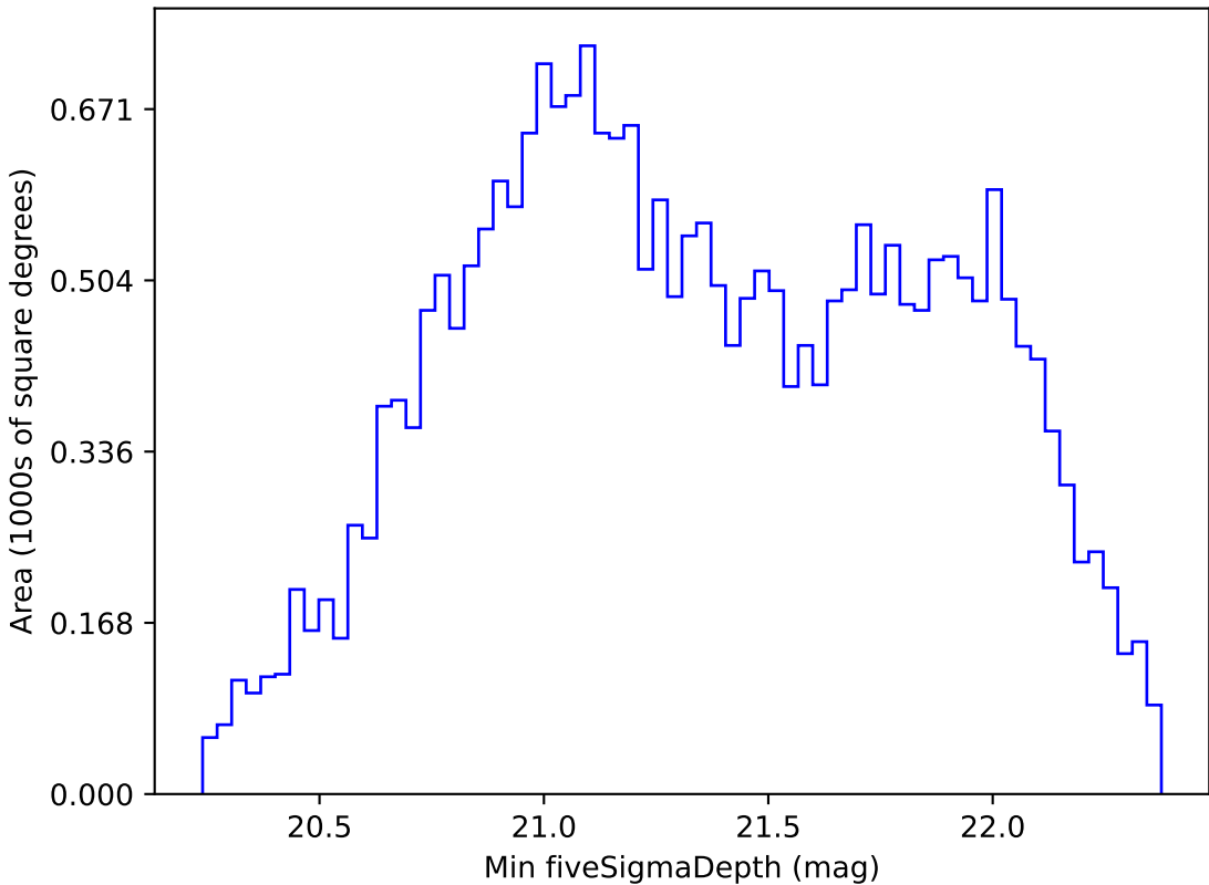
weather_cloudso4v3.4_10yrs All sky z band: Min fiveSigmaDepth
