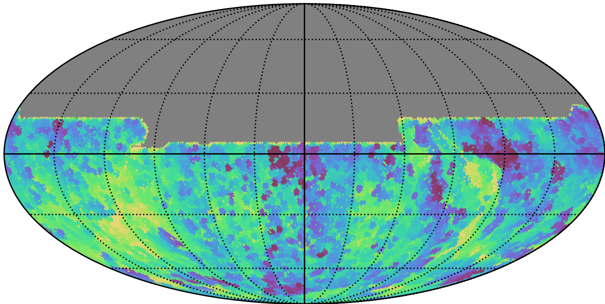
weather_cloudso4v3.4_10yrs All sky y band: Min fiveSigmaDepth
