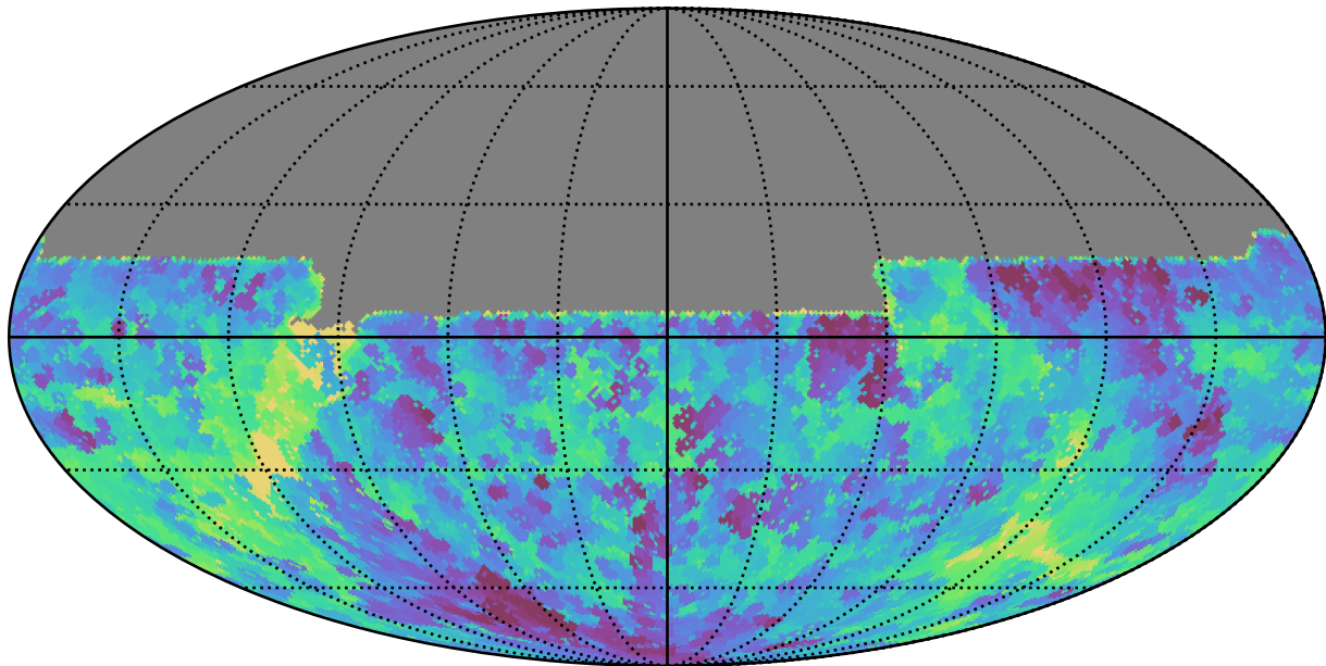
weather_cloudso4v3.4_10yrs All sky u band: Min fiveSigmaDepth
