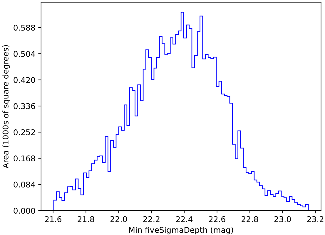
weather_cloudso4v3.4_10yrs All sky u band: Min fiveSigmaDepth
