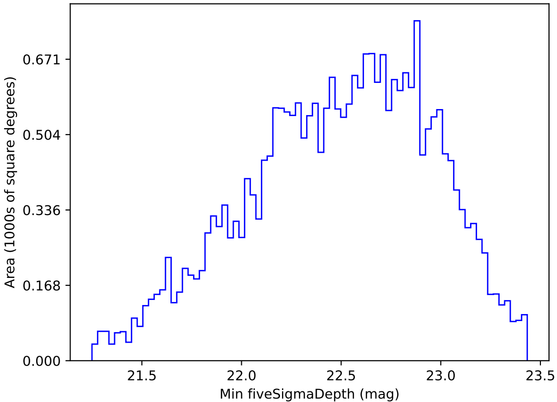
weather_cloudso4v3.4_10yrs All sky r band: Min fiveSigmaDepth
